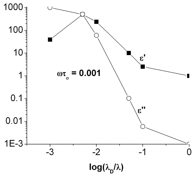
Figure 6: Dependences of \epsilon'(\omega\tau_\sigma) and \epsilon''(\omega\tau_\sigma) on \frac{\lambda_D}{\lambda} , for (\omega\tau_{sigma})=10^{-3}
