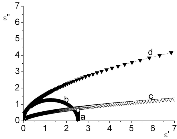
Figure 5: Nyquist diagrams \epsilon''(\omega\tau_\sigma) = f(\epsilon'(\omega\tau_\sigma))_T
