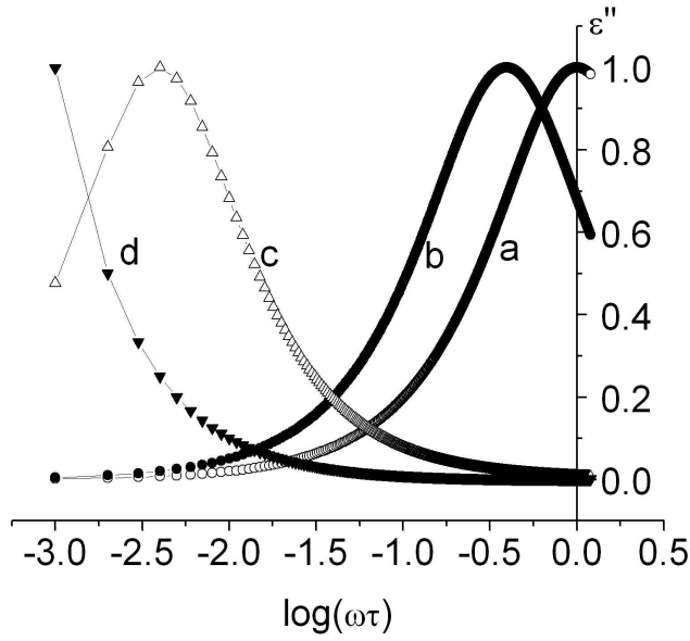
Figure 4: The dependences \epsilon''(\log \omega \tau_{\sigma}) . The values are normalized at \epsilon''_{max}
