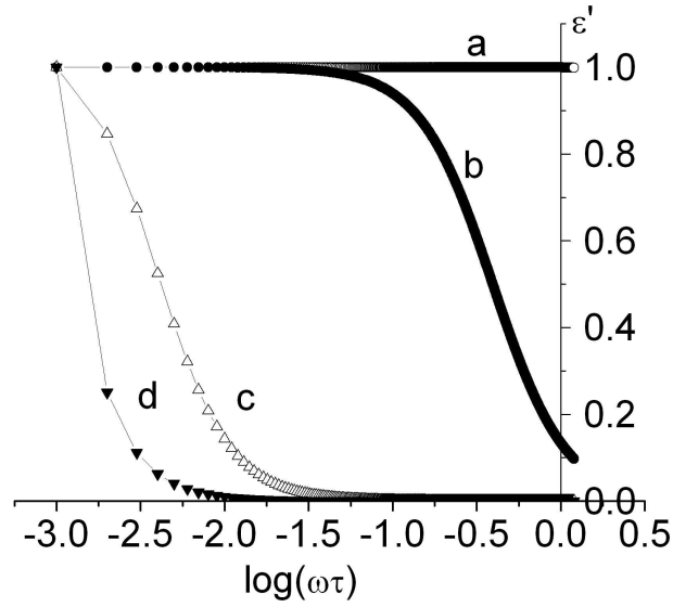
Figure 3: The dependences \epsilon'(\log \omega \tau_{\sigma}) . The values are normalized at \epsilon'_{max}
