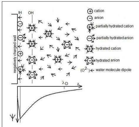
Figure 2: EDL structure for p-Si (SCL negative charged, \epsilon_F < \epsilon_{FR} )/aqueous solvent interface. The electrostatic potential and charged atoms in solvent distributions vs the distance z from the wall.
